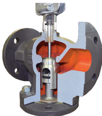
Sectional view of bælz 340-B-EMF-2 plug
