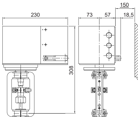
Dimensions of the bælz 373-E65 actuator
